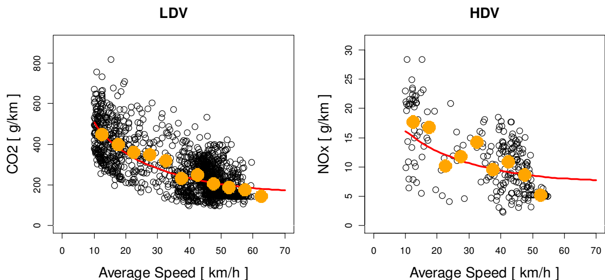
Figure 4: Comparison of CO 2 and NO x emission factors, COPERT Australia (Line) and Aimsun – PΔP (Black Dot Points, Yellow Points are mean values for 5 km/h speed bins)
